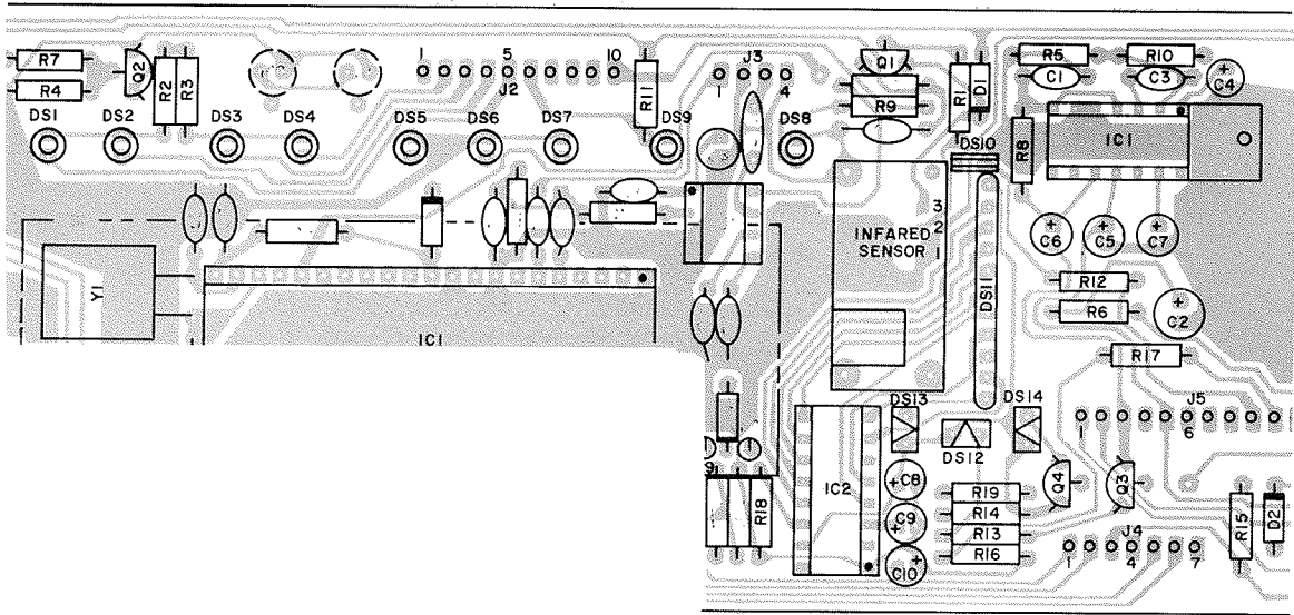
CONTROL/DISPLAY PCB 046906
